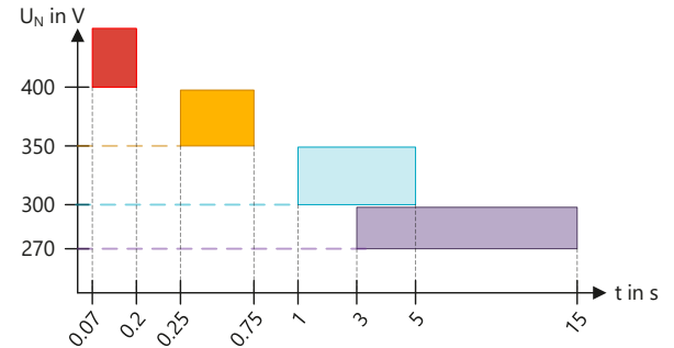
Voltage time window from EN 50550 within which a POP main protective device must trip.
